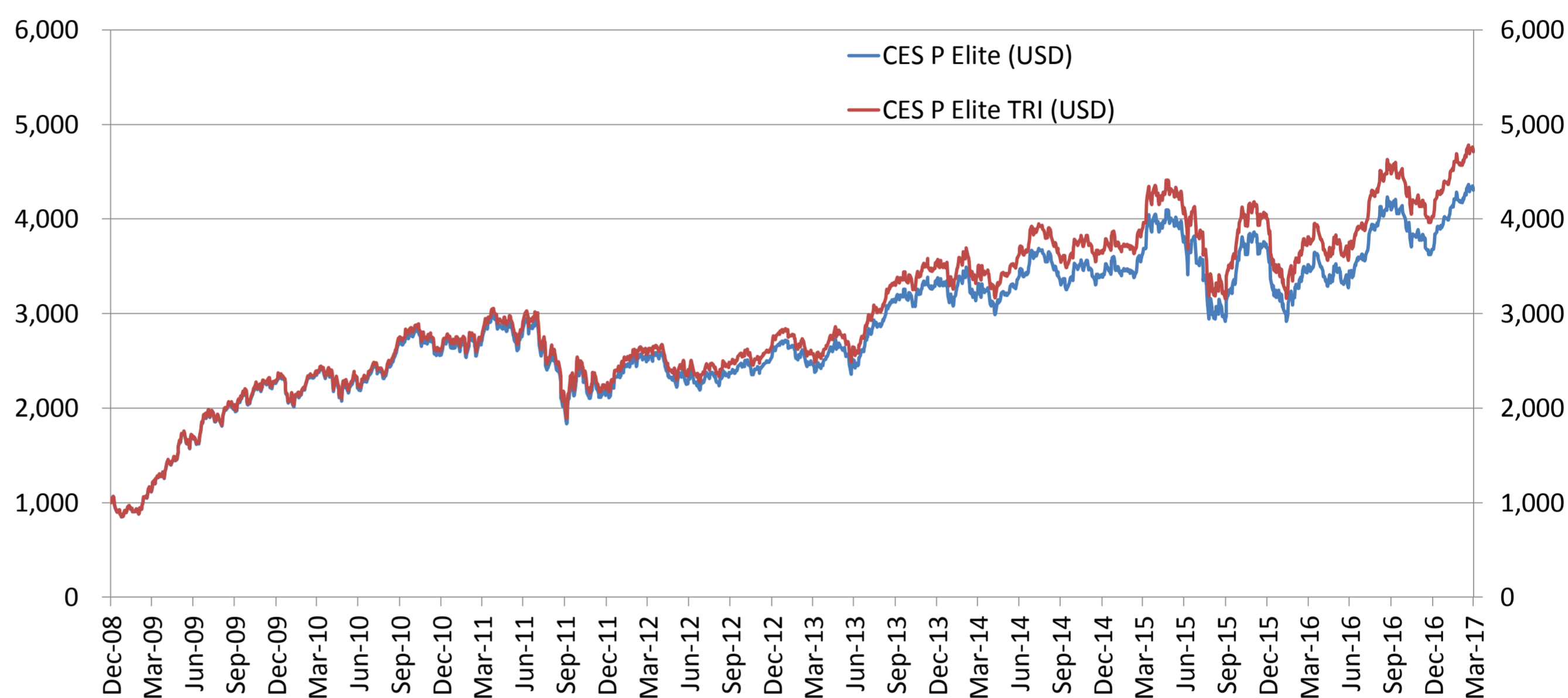
TRI-Total Return Index Source: CESC, CSI as at 31 Mar 2017
